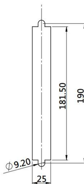
PANEL CUTOUT
